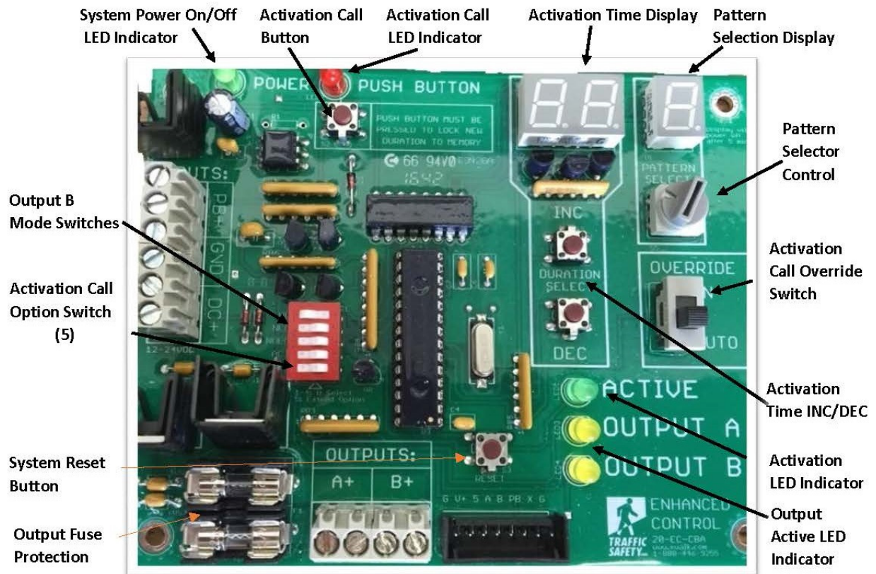
Enhanced Control Board
